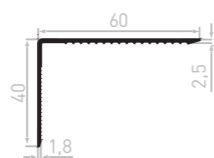
CE2530C_AL Corner angle 60 x 40x2.5-2 Alu Serrated 5 bars of 6 ml / pack
