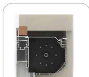
Renovation installation
