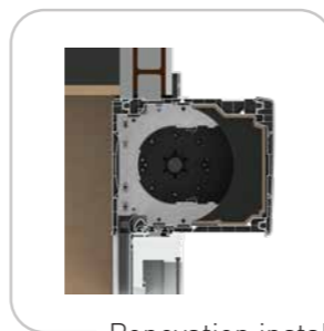
Renovation installation
