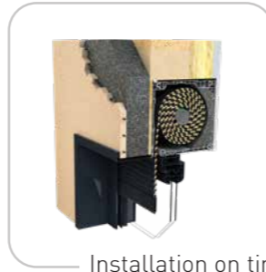
Installation on timber- frame house
