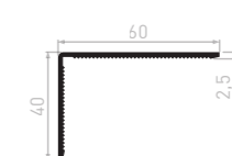
CE2530C Corner angle 60x40x2,5 Serrated 10 bars of 6 ml / pack 600 bars of 6 ml / container
