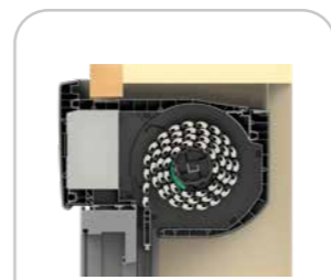
Renovation installation
