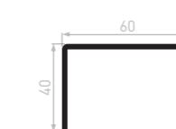
CE2530 Corner angle 60x40x2,5 10 bars of 6 ml / pack 500 bars of 6 ml / container
