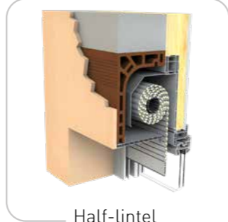
Half-lintel installation
