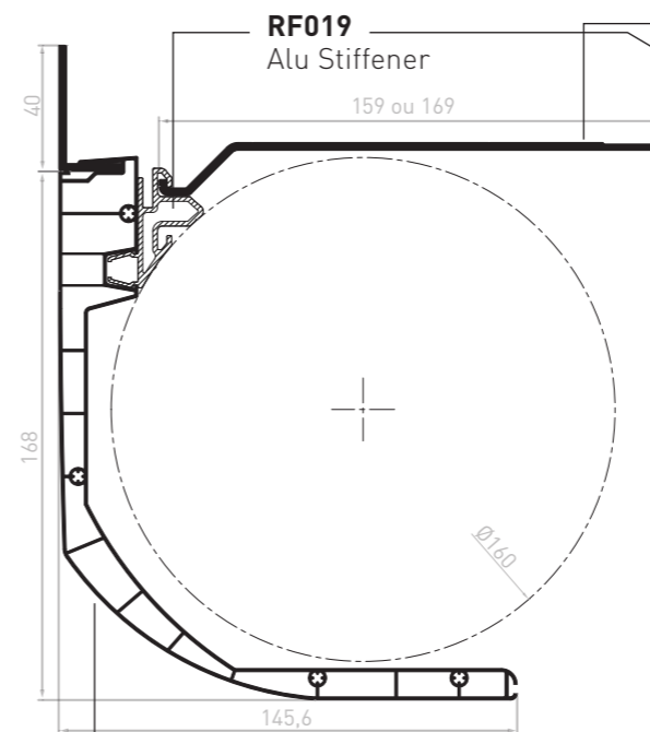
VR063F Front plank
