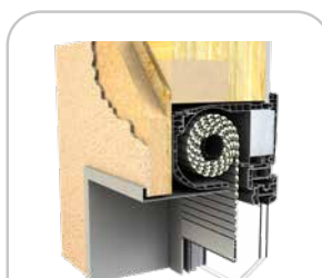
Installation on timber-frame house
