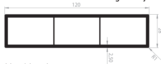
CL003 - 120x28 - R1 for hanger only
