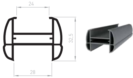
CL010 - Filling moulding 24/28mm
