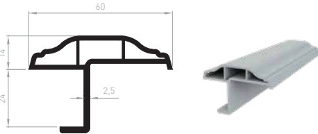
CL042 - Moulding 24MM
