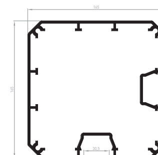
CL127_AL Post 165x165
