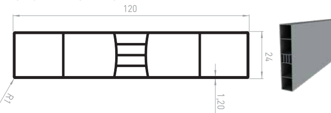
CL029 - Bar 120x24MM
