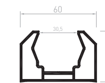
CL099_AL Post 1 slots 60x40
