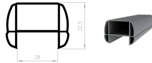
CL011 - Mortise moulding 28mm
