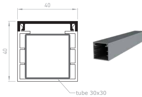
CL031 - Tube sheathing 30x30MM
