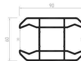
CL084 Post 2 slots 90 x 60
