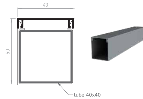
CL030 - Tube sheathing 40x40MM
