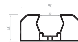
CL061 Post 1 slots 90x40
