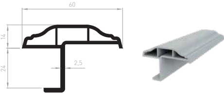
CL041 - Moulding 24MM
