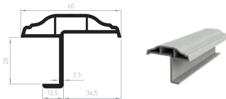
CL066 - Moulding 28MM
