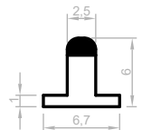
AC119_N0004 Joint gomme noir 6,7 x 6 mm
