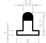
AC103_N0004 Joint gomme noir 5 x 5,1 mm
