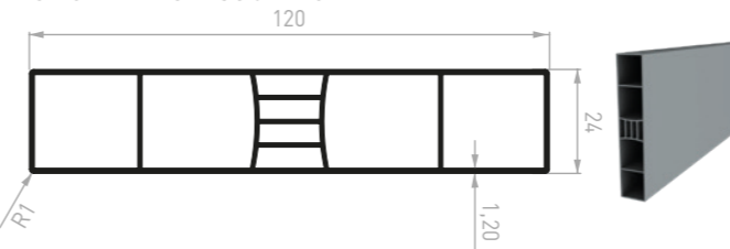
CL029 - Barreau 120x24MM
