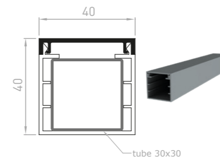
CL031 - Gainage tube 30x30MM
