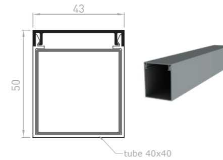
CL030 - Gainage tube 40x40MM
