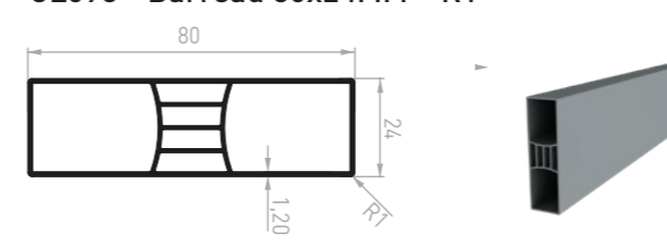
CL098 - Barreau 80x24MM - R1
