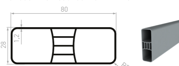
CL005 - Barreau 80x28MM - R5
